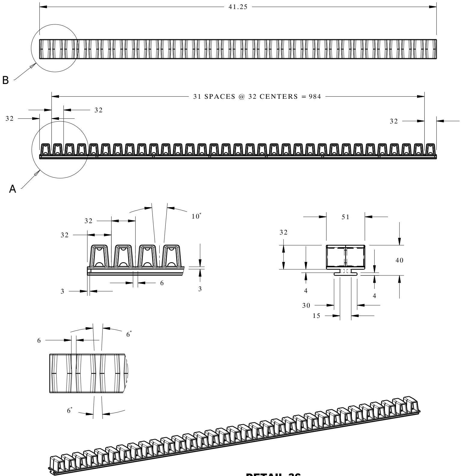
DETAIL 36
