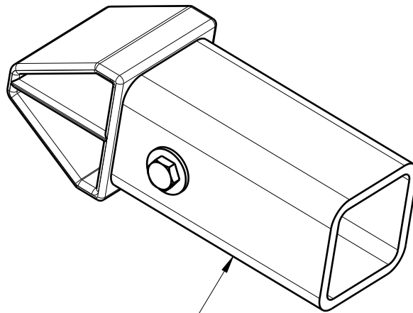
2.00" SQ. 7GA. TUBE SHOWN FOR REFERENCE
