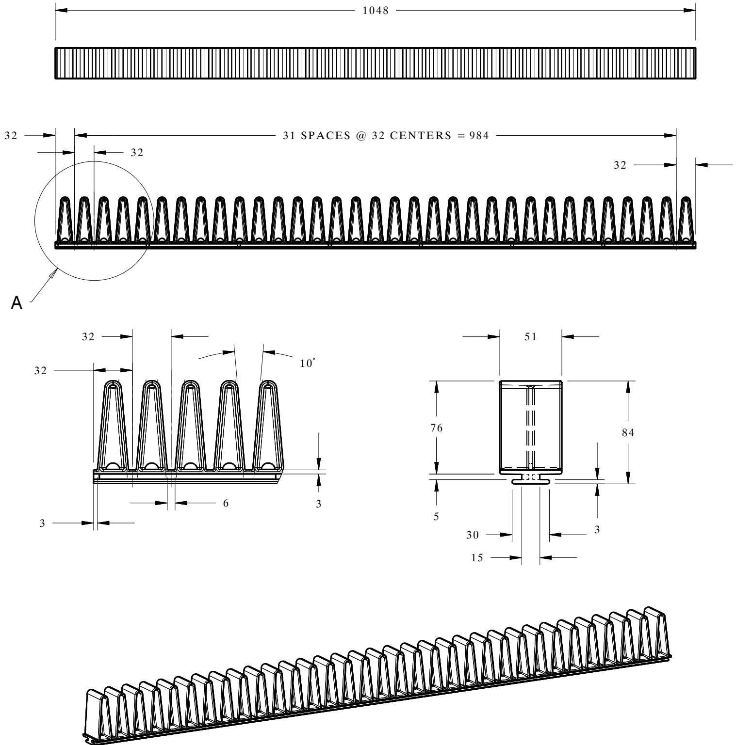
DETAIL 37
